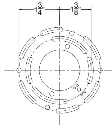
Mounting Hole Dimensions
