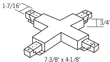
"X" Connector
