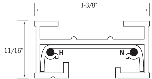
Grooved Polarity Line
