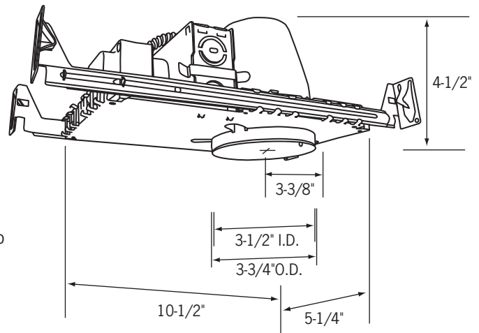
Ceiling Opening: 3-7/8" Max. Ceiling Thickness: 1/2" - 1-1/4"
