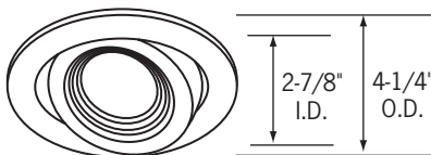
CTR306-P Surface Adjustable; Black Baffle 40° Vertical adjustment, 359° horizontal rotation. 50mm Lens. Regressed black baffle reduces surface brightness. Flat, stainless mounting clips hold trim firmly to ceiling. Trim can hold up to two (2) lenses with stepped lens holder (included). Insert 45mm lens on lower level of lamp seat, insert 50mm lens onto higher level.
