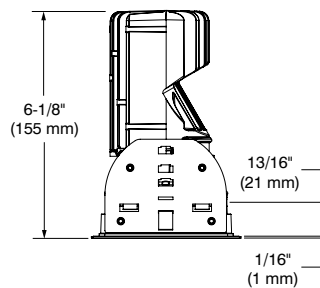
WITH FLANGE
