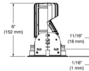
WITH FLANGE
