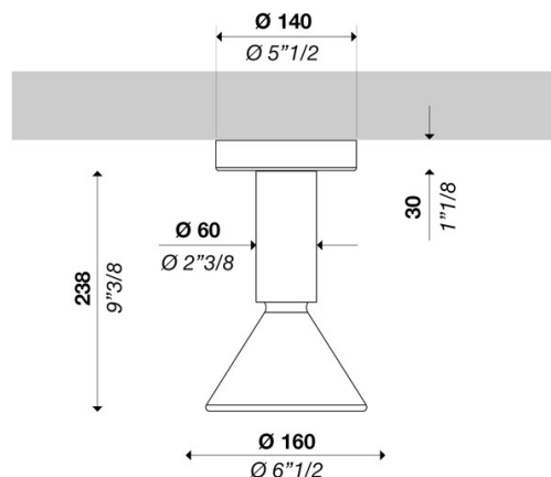
Technical drawing Size ref. image mm - inch
