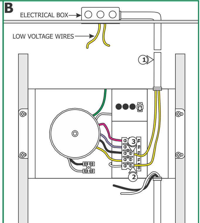
TERMINAL TAP CHART
