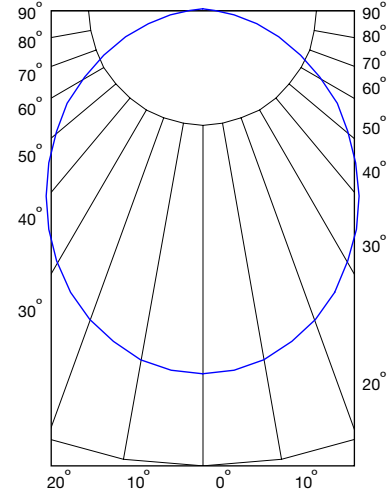
CANDLE POWER DISTRIBUTION 105°
