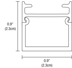
CIRRUS CEILING S1 SQUARE LENS (ACTUAL SIZE)
