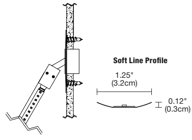
Non-Power Feed Turnbuckle Included with SLT-SA
