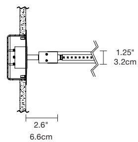
Power Feed Turnbuckle Included with SLT-SA
