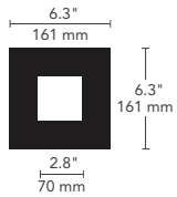
FLANGED
