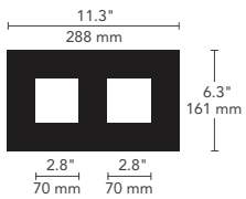
FLANGED
