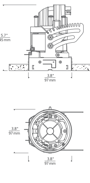
*SHOWN IN ROUND FLANGED AT NO TILT (0°)
