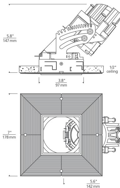
*SHOWN IN SQUARE FLANGELESS AT FULL TILT (45°)
