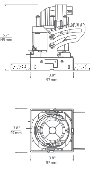
*SHOWN IN SQUARE FLANGED AT NO TILT (0°)
