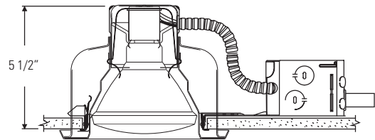
1084/1003R Lytefiring™ Non-IC Remodeler
