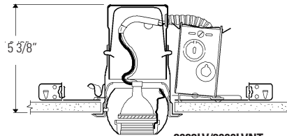
2022LV/2000LVNT Remote Transformer Low Voltage
