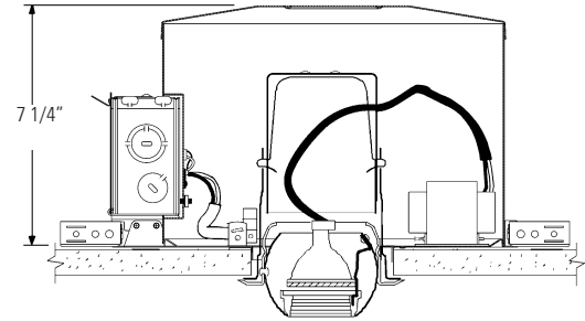
2022LV/2004ICV/N LyteSeal™ AirSeal® Insulated Ceiling
