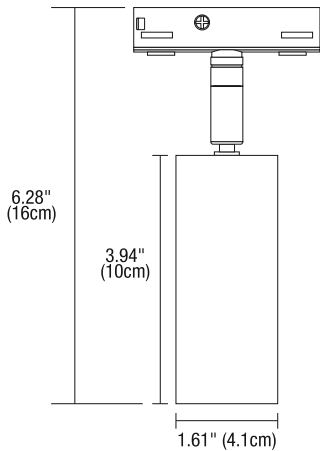
T24M-2C-TUBS-SP-30K-BK
