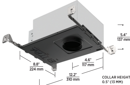
IC AIRTIGHT/FIRE-RATED CHICAGO PLENUM
