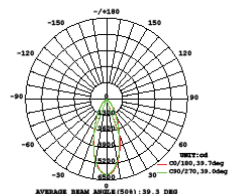
8" Diameter, 3000K, Straight Up or Down Distribution
