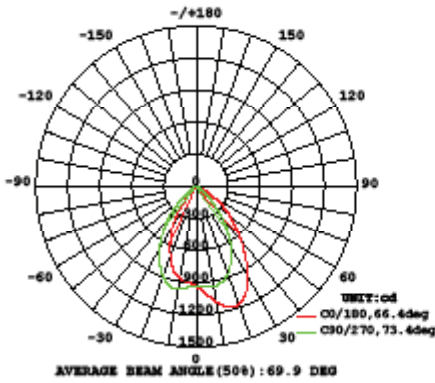
5" Diameter, 3000K, Away From or Towards Wall Distribution
