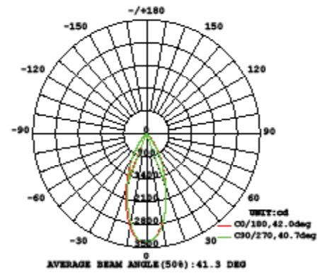
6" Diameter, 3000K, Straight Up or Down Distribution
