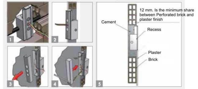
Assembly instructions for outer casing masonry wall
