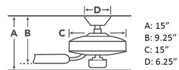
With 4.5" Downrod
