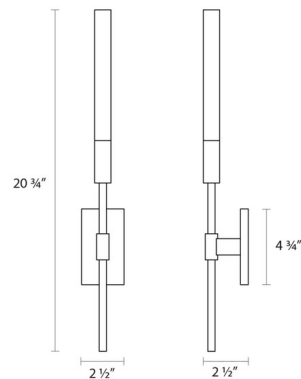
Shown in bright satin aluminum / frosted
