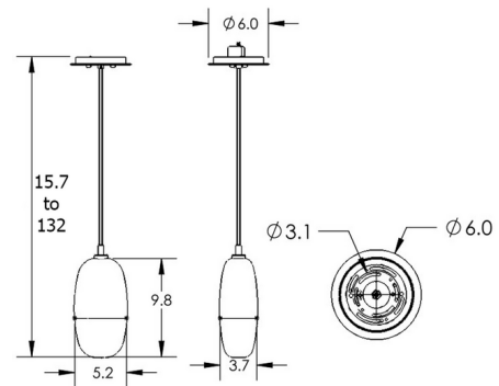
Mounting Method: J-Box Ceiling Mount, Minimum J-Box Size Requirement is 4" W, 4" L, 1.5" D
