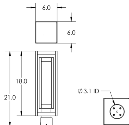
Mounting Method: Mounts Directly To Post
