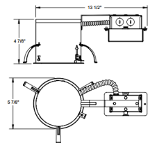
5 1/2" CEILING CUTOUT
