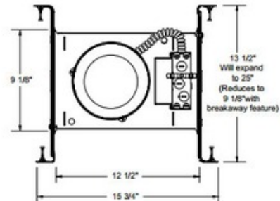
6 7/8" CEILING CUTOUT
