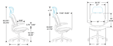
Freedom Task Chair with Headrest
