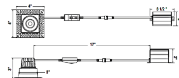
2in Square 8W Trimless Downlight
