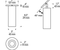
Surface Mount Canopy:
