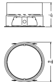
ED1-TC2 Thick Ceiling Adapter for ceilings 1 5/16" to 2"
