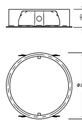
ED1-TC1 Thick Ceiling Adapter for ceilings 11/16" to 1 1/4"
