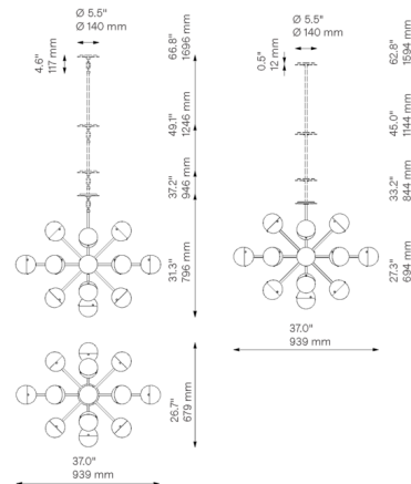
Shown in lacquered burnished brass / sand blasted
