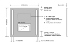
DIMENSIONAL DRAWING (Not to scale. Front and border widths may vary depending on mirror size.)
