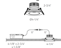
GBR35-DW - 3.5" Dim-To-Warm Regressed Gimbal Downlight
