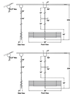
Shown in antique-burnished brass / seeded glass
