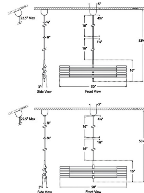
Shown in antique-burnished brass / seeded glass
