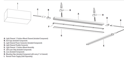
Included Components: Indoor Light Channel .3 Surface Mount system overview
