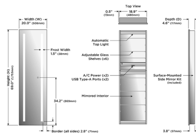
DIMENSIONAL DRAWING (not to scale)
