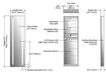
DIMENSIONAL DRAWING (not to scale)
