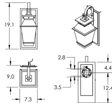
Mounting Method: J-Box Wall Mount
