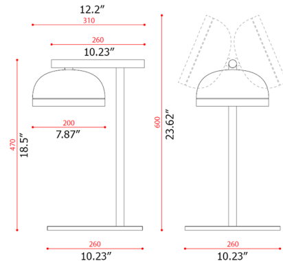
Shown in brushed brass ring / brushed brass dome
