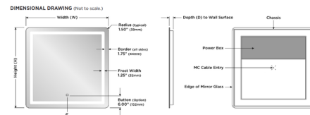
Dimensions 36" W x 36" H x 1.75" D (36mm W x 36mm H x 44mm D)
