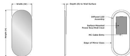
DIMENSIONAL DRAWING (Not to scale)
