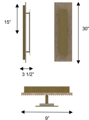
Shown in painted antique brass / travertine
