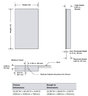
DIMENSIONAL DRAWING (Not to scale)
