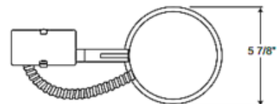
5 1/2" CEILING CUTOUT
