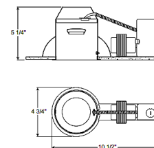
4 3/8" CEILING CUTOUT
