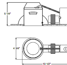
4 3/8" CEILING CUTOUT
