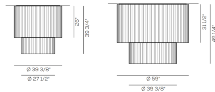
INTERNAL DIFFUSER
