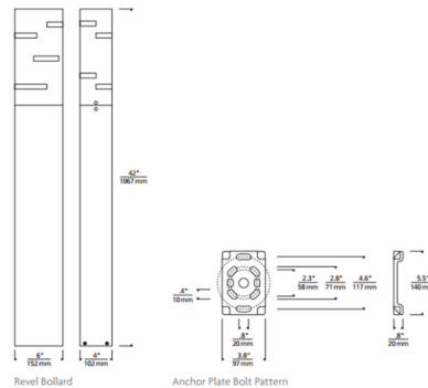
Revel Bollard
