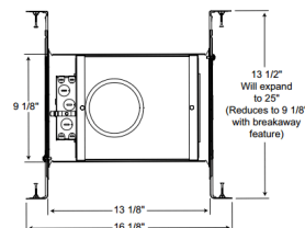
4 1/2" CEILING CUTOUT
