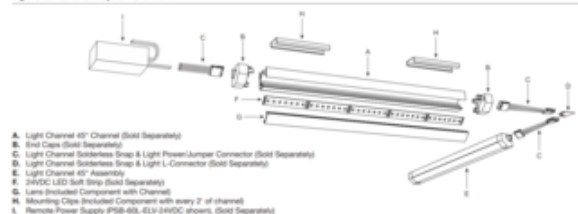
Light Channel 45° DIY System Overview
