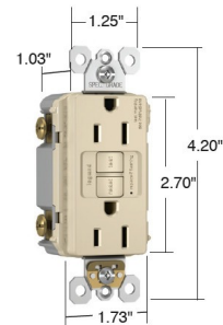
Dimensions for 15 & 20 Amp
