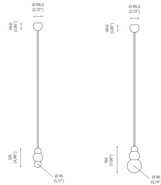
120V version supplied with paintable junction box cover.
