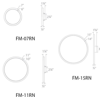
Driver installed within the Junction Box, driver dimension: 2.25" Dia x 1" Deep
